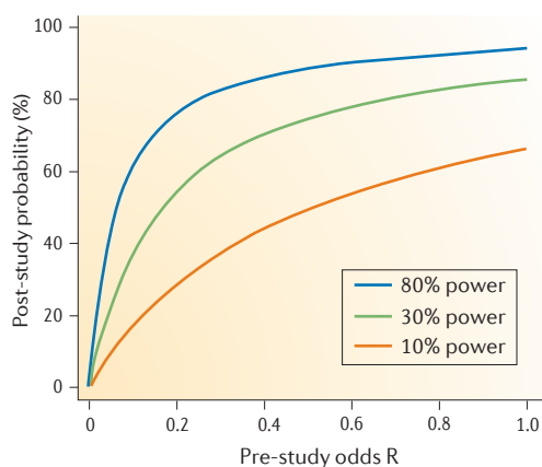
Figure 4 | Positive predictive value as a function of the pre-study odds of association for different levels of statistical power.
